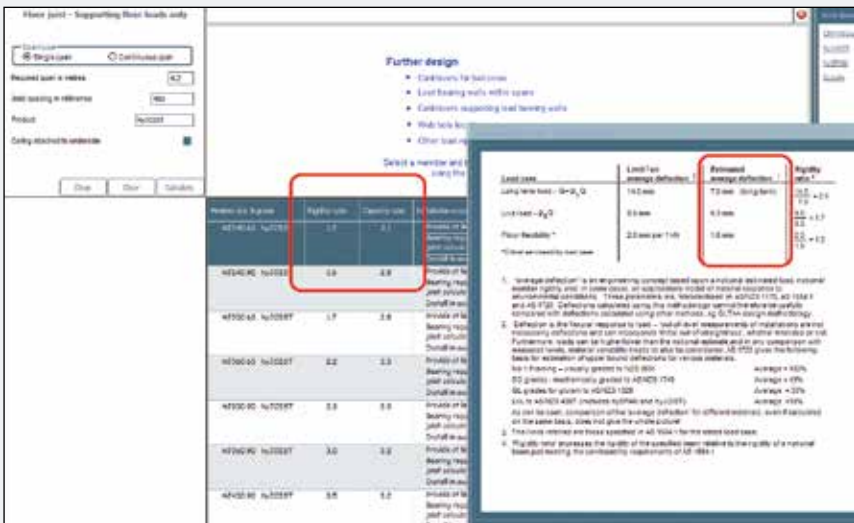
Figure 1: Rigidity and Capacity Ratio's and Estimated Average Deflection
